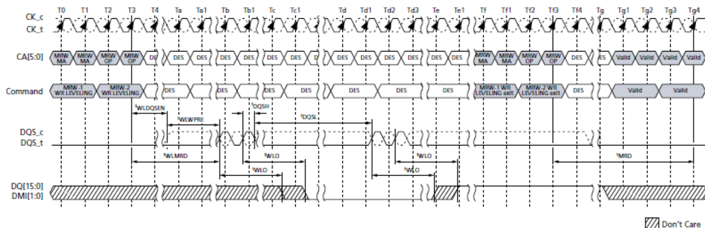
Write Leveling Timing – t_{DQSL}(\text{MAX})
