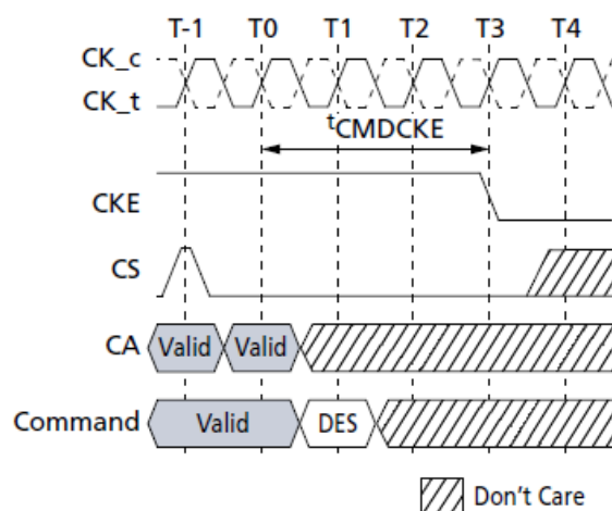
t_{CMDCKE} Timing
