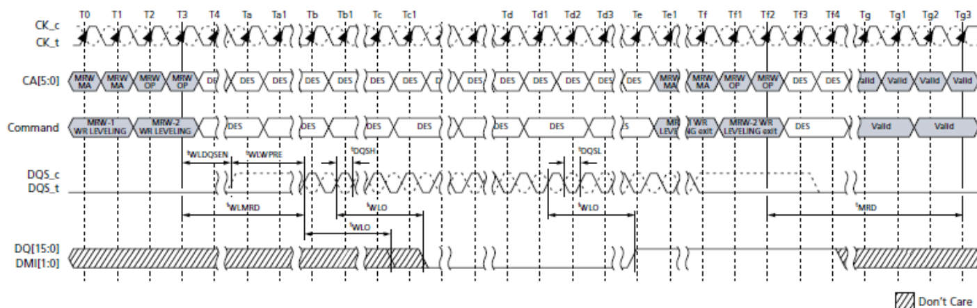
Write Leveling Timing – t_{DQSL}(\text{MIN})
